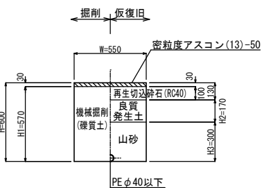
㉚ 宅地内 (As)
